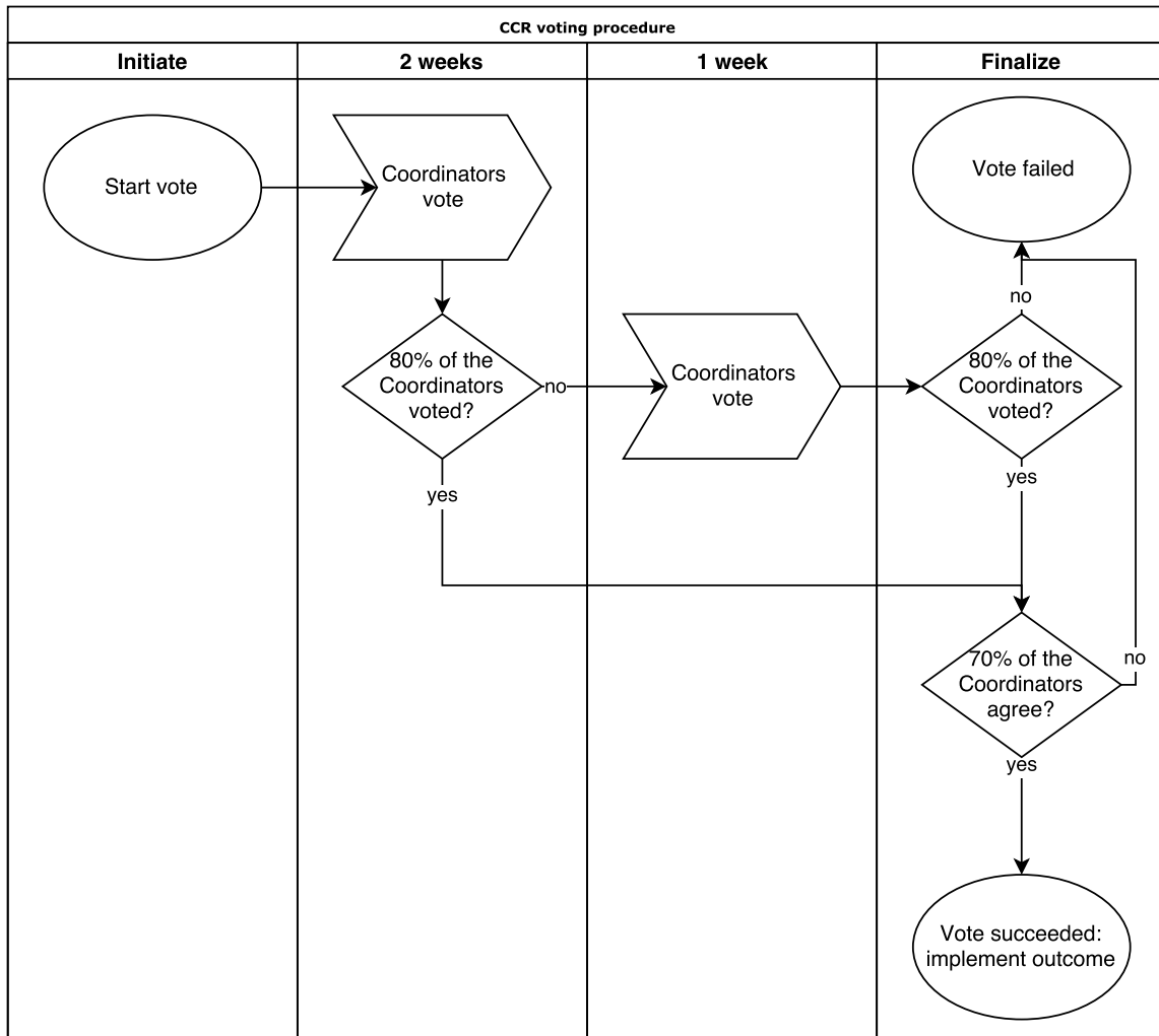
Figure 1.1: CCR voting procedure.
