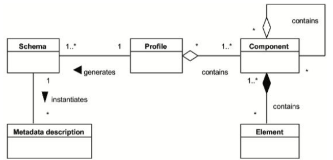
Figure 8.1: Component Metadata model (ISO 24622-1, 2015).
